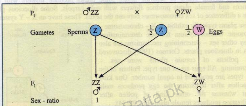
Fig. 22.22 Sex determination in birds and butterflies.
