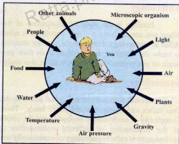
Fig. 25.1 Your environment
