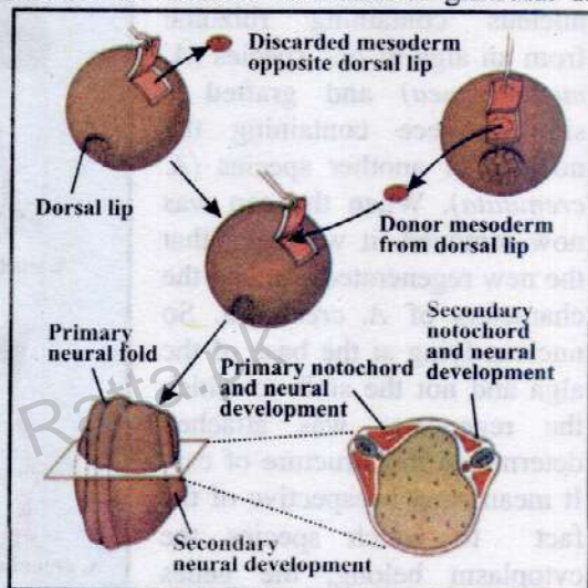
Fig. 19.11 The Spemann primary organizer experiment.
