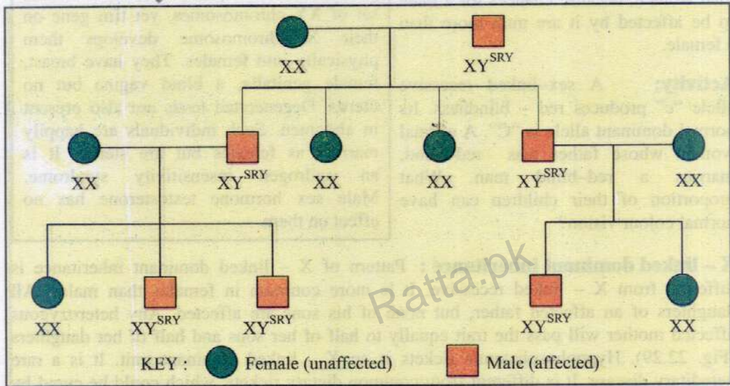
Fig. 22.30 Y-linked inheritance in man.
