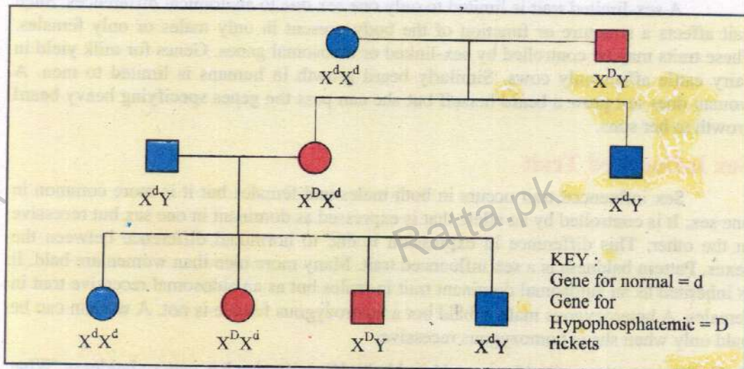
Fig. 22.29 Transmission of X-linked dominant trait in humans.
