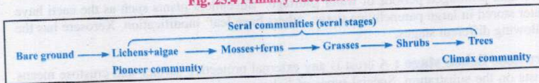
Fig. 25.4 Primary Succession
