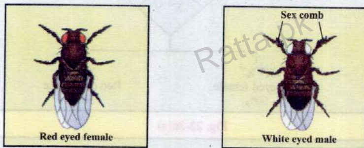
Fig. 22.25 Wild type red eyed female and mutant white eyed male Drosophila .
