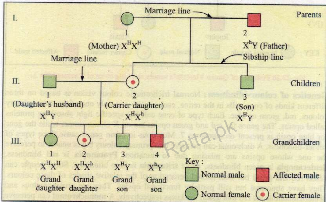
Fig. 22.27 Transmission of X-linked recessive trait (haemophilia) in humans.
