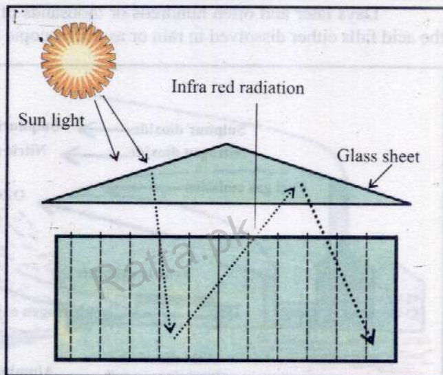
Fig. Greenhouse effect
