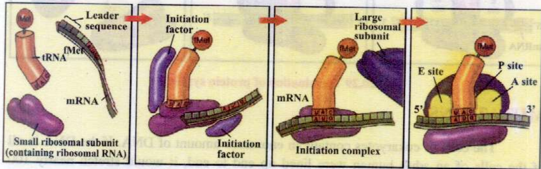
Fig. 20.27 Formation of the initiation complex.
