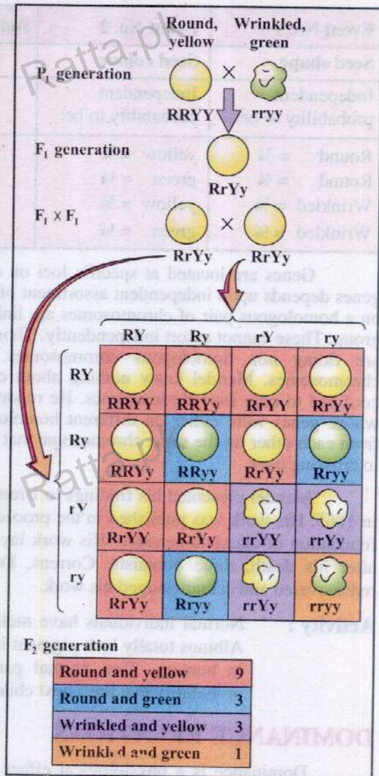
Fig. 22.6 Dihybrid cross produces parental as well as recombinant types.
