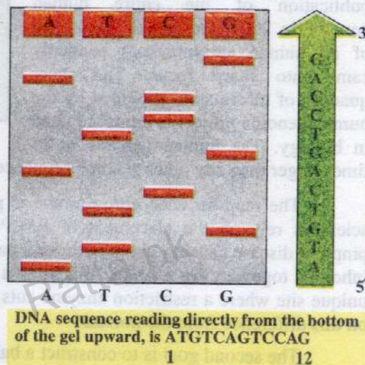
Fig. 23.8 The enzymatic or dideoxy method of sequencing DNA .
