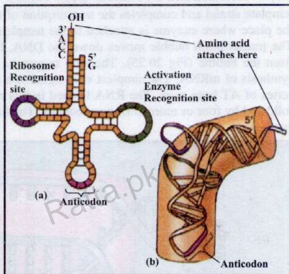
Fig. 20.24 The structure of tRNA (a) two-dimensional schematic (b) three dimensional structure.
