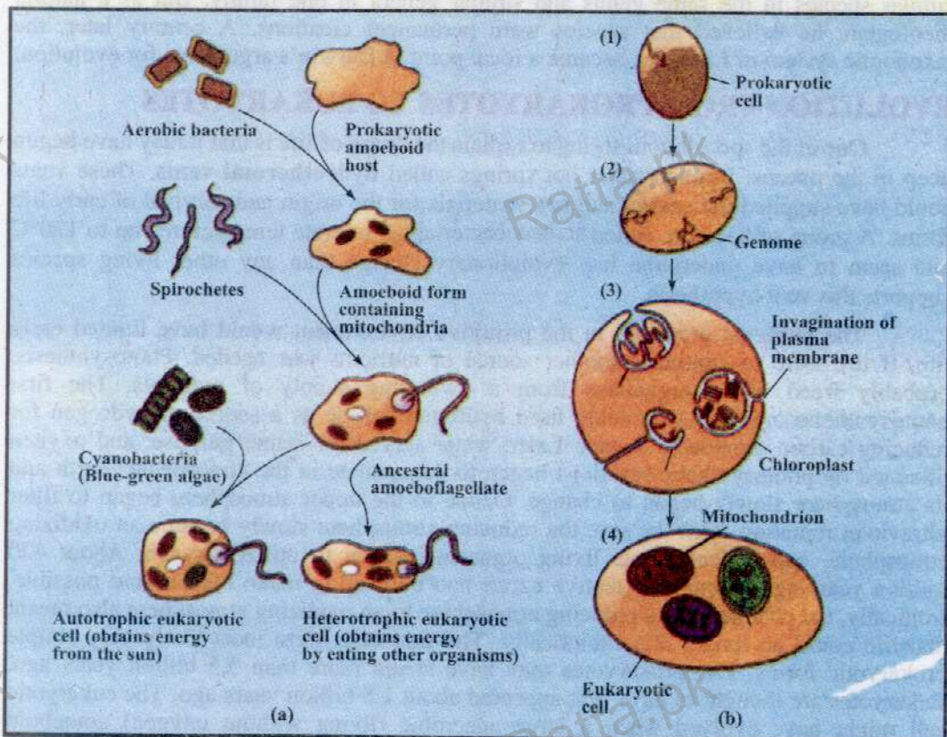
Figure 24.1: Two hypotheses on the evolution of the eukaryotic cell. (a) Endosymbiont hypothesis, (b) Membrane invagination hypothesis. (1) A prokaryotic cell (2) Duplicates its genetic material (genome) (3) The plasma membrane then invaginates to form double membrane-bound organelles, and the individual genomes separate from each other (4) The nuclear genome eventually enlarges, while the other organelle genomes lose many of their genes, resulting in a eukaryotic cell.
