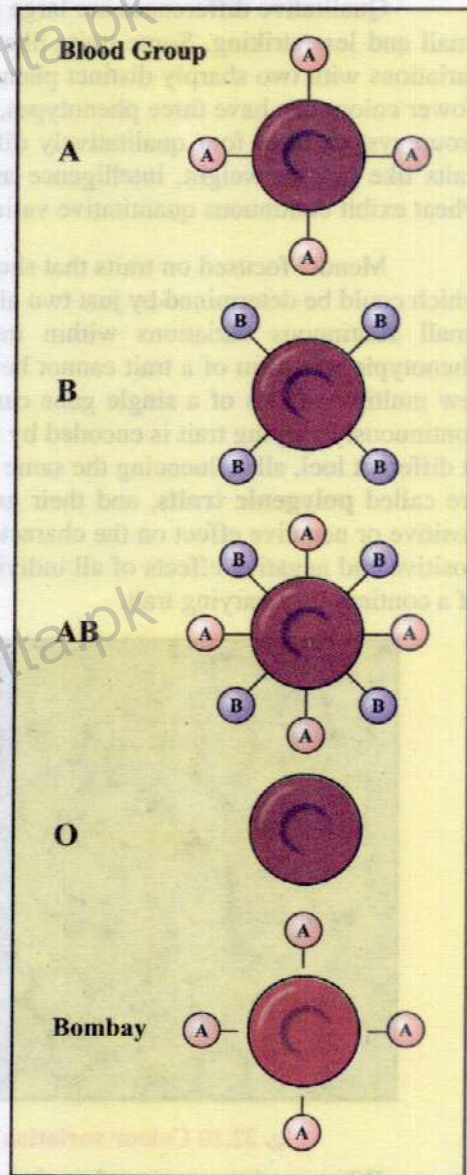
Fig. 22.9 Bombay phenotype results from epistasis
