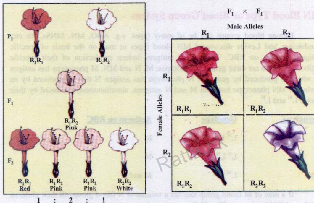
Fig. 22.7 Incomplete dominance in 4 O'clock
