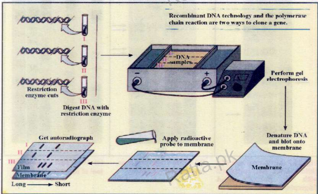
Fig. 23.6 DNA fingerprinting. Three samples of DNA (I, II, III) were cut with a restriction enzyme and run on agarose gel. The gel pattern was then transferred to a membrane and DNA was denatured. The denatured DNA on the paper was hybridized with radioactive probe. Since the radioactive probes had complementary arrangement of bases to the original DNA, all DNA fragments were labelled, which appeared as black bands with autoradiogram.
