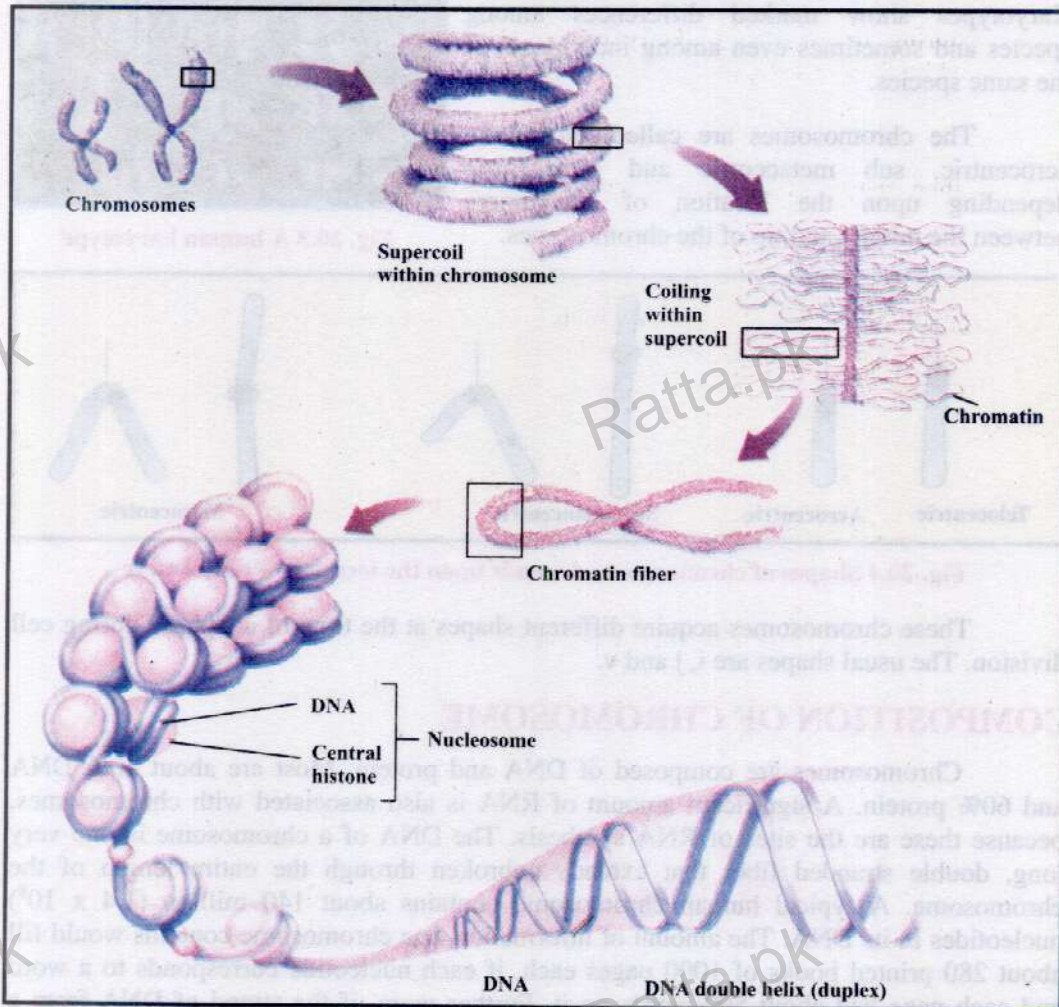
Fig. 20.5 Levels of eukaryotic chromosomal organization.
