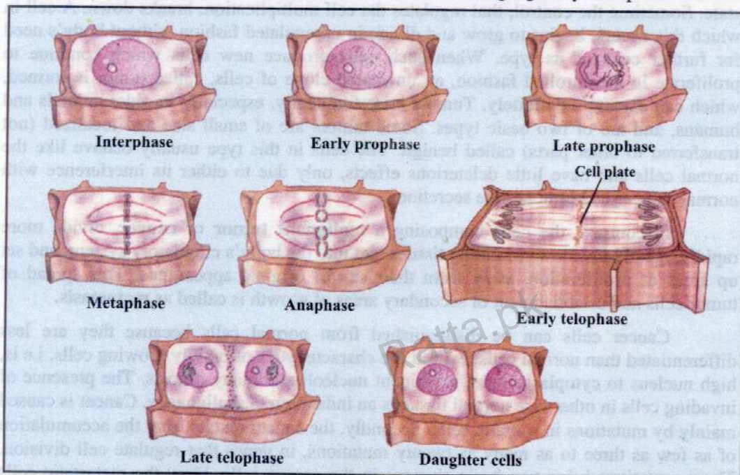
Fig 21.3 Mitosis in a higher plant cell
