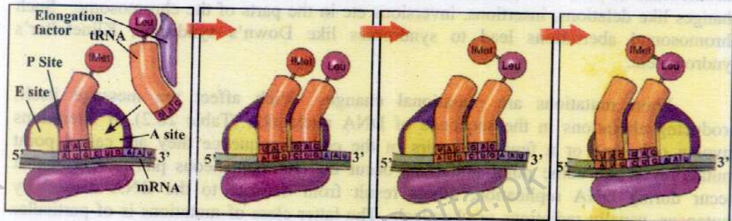
Fig. 20.28 The translocation process.
