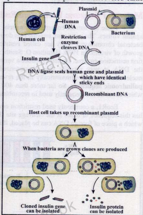
Fig. 23.2 Cloning of a gene.
