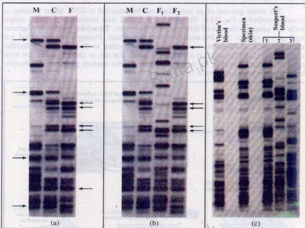
Fig. 23.7 (a) Comparison of a child's DNA fingerprint (c) with his parent's DNA fingerprints (M and F).
