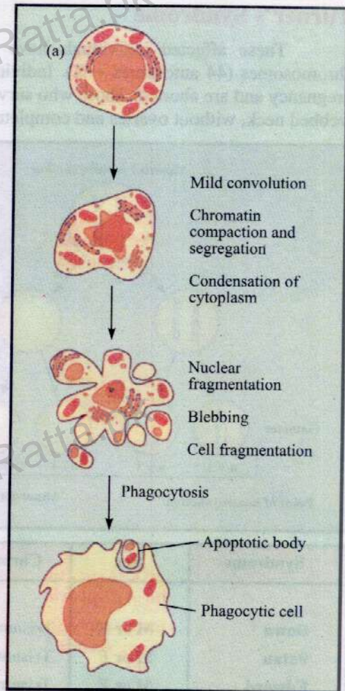
Fig21.7 Ultrastructural features of cell death by apoptosis
