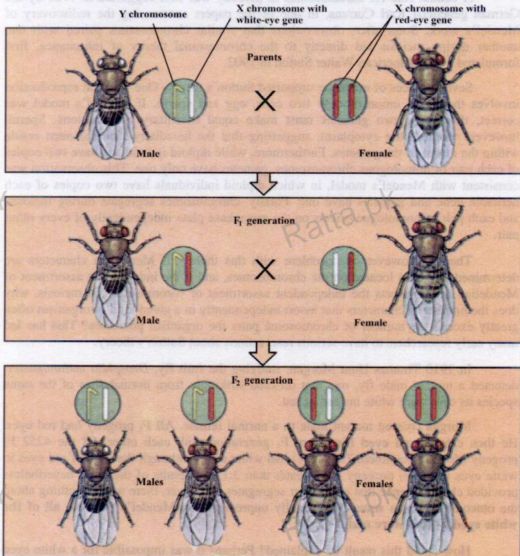
Fig. 20.6 Morgan's experiment demonstrating the chromosomal basis of sex linkage.
