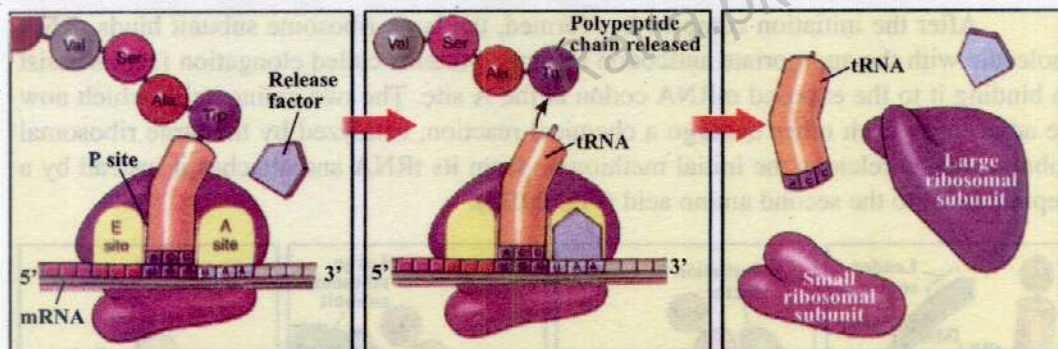
Fig. 20.29 Termination of protein synthesis
