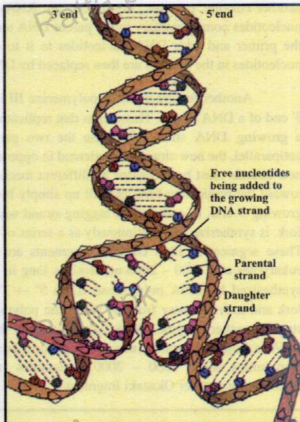
Fig. 20.17 Replication of DNA
