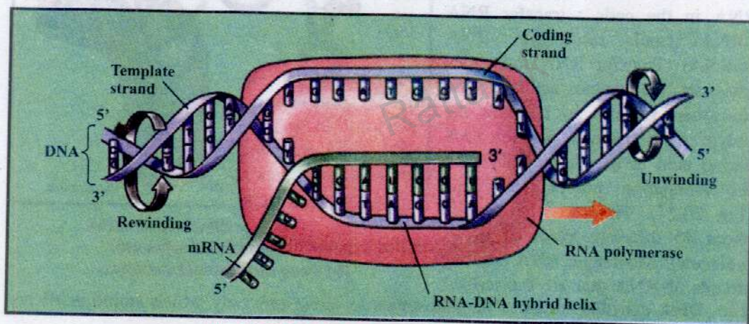
Fig. 20.25 Model of a transcription bubble.
