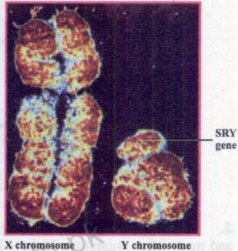
Fig. 22.19 Sex Chromosomes of a man.
