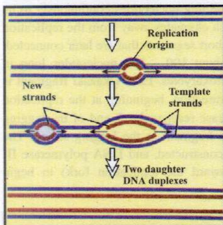
Fig. 20.16 Origins of replication.
