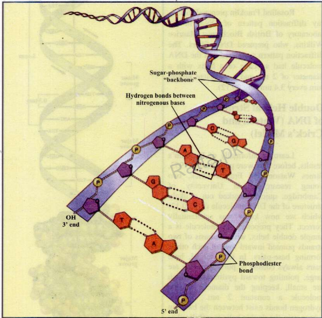
Fig. 20.13 DNA is a double helix.
