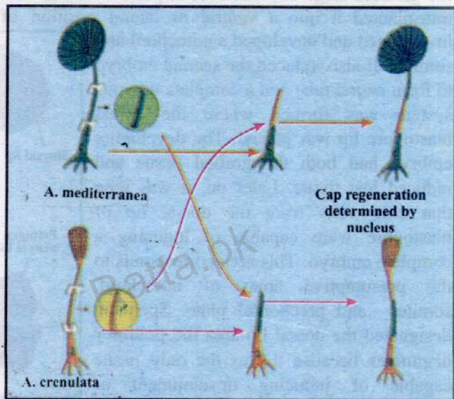
Fig. 19.10 Nuclear control of cap structures in two species of Acetabularia .
