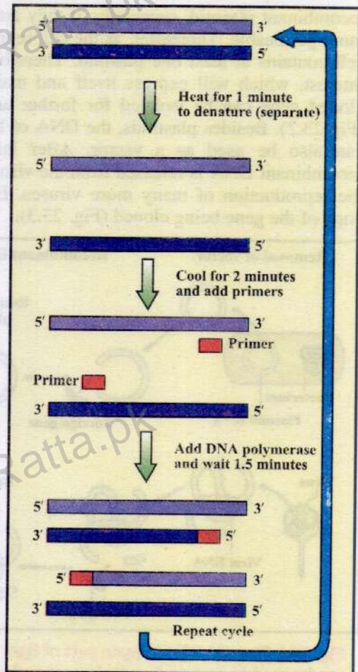
Fig. 23.5 Polymerase chain reaction (PCR).
