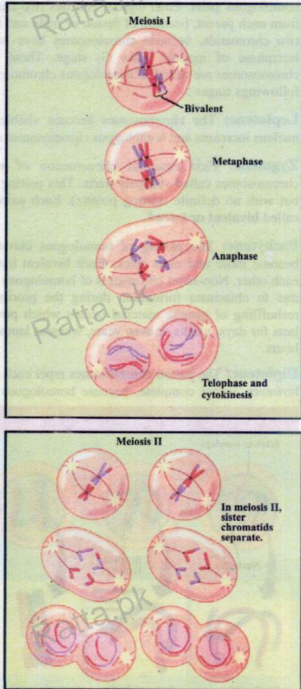
Fig 21.4 Result of meiosis, four haploid cells, each with half as many chromosomes as the original cells
