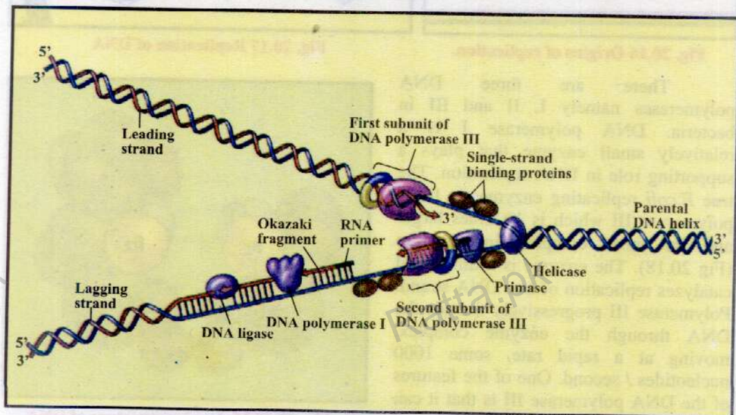
Fig. 20.19 A DNA replication fork.
