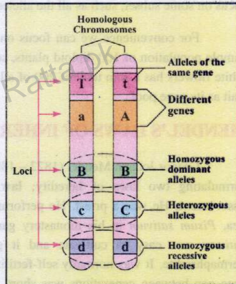
Fig. 22.1 Allelic pairs on a homologous pair of chromosomes
