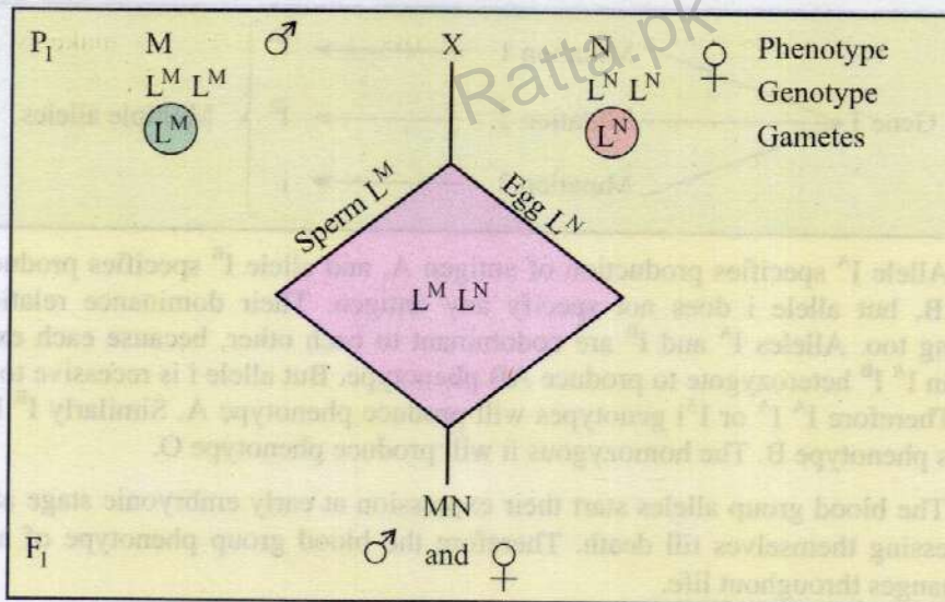
Fig. 22.8 Codominance in MN Blood group alleles.
