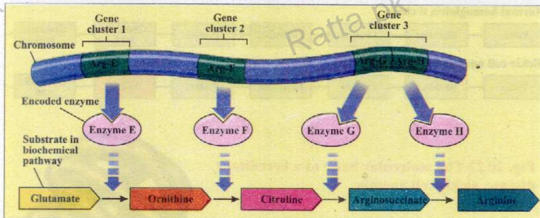
Fig. 20.21 Evidence for the “one-gene/one-polypeptide” hypothesis.
