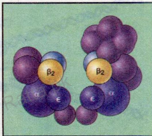
Fig. 20.18 Molecular structure of DNA polymerase III complex.
