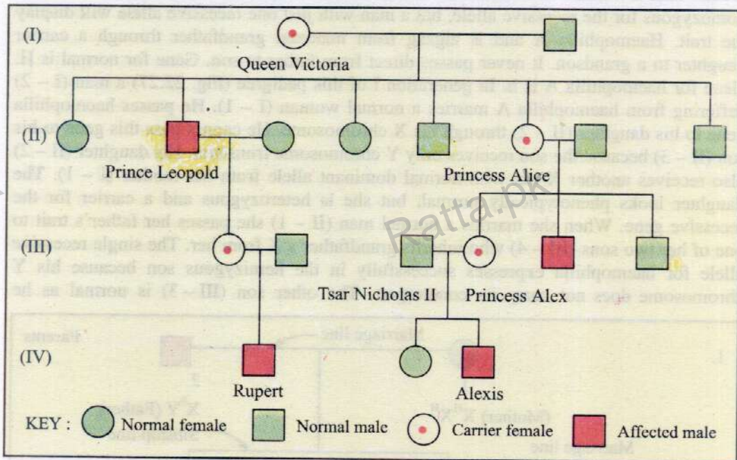
Fig. 22.28 Pedigree of Queen Victoria's family showing cases of Haemophilia A.
