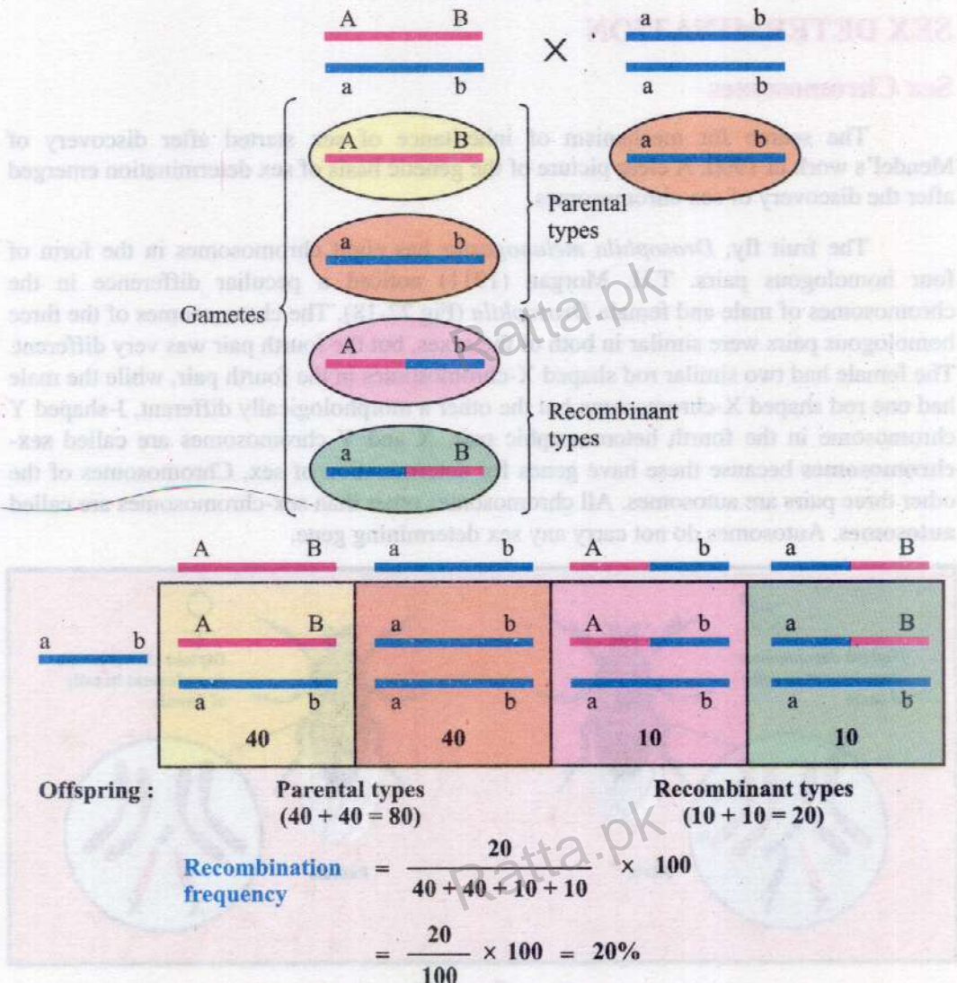
Fig. 22.17 Recombination frequency between two linked genes.
