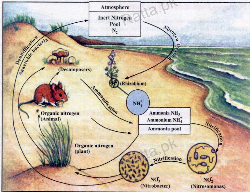
Fig. 25.5 Nitrogen cycle
