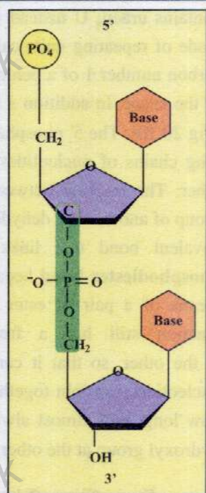
Fig. 20.11 A Phosphodiester bond.
