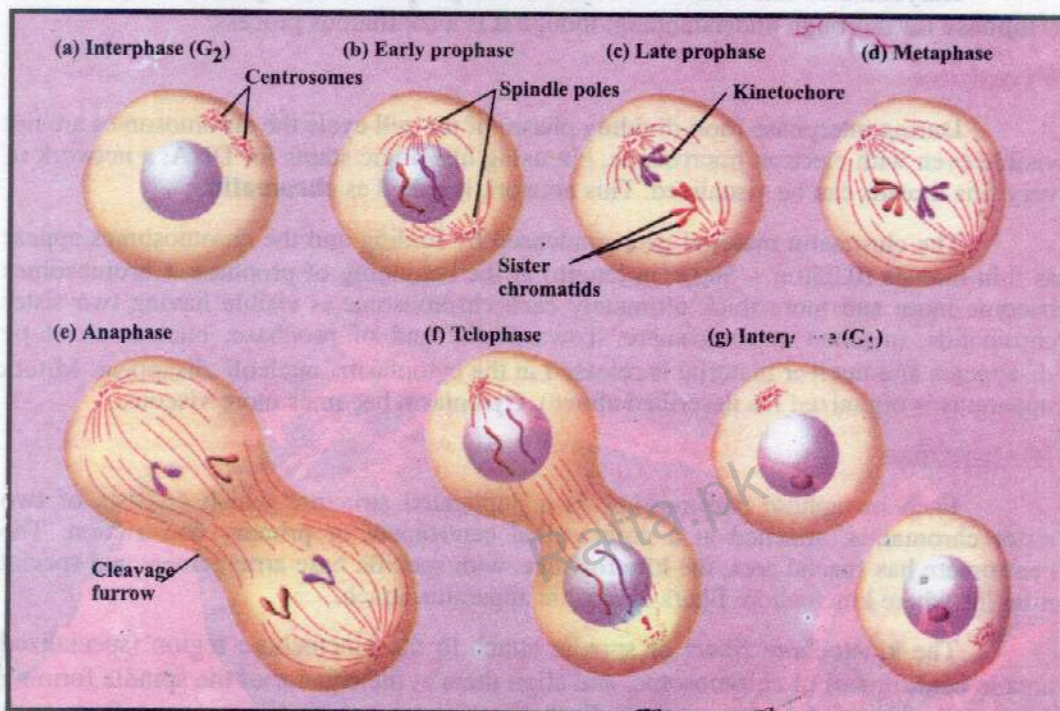
Fig 21.2 The stages of mitosis and cytokinesis in an animal cell.
