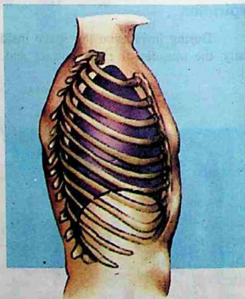
Expiration
