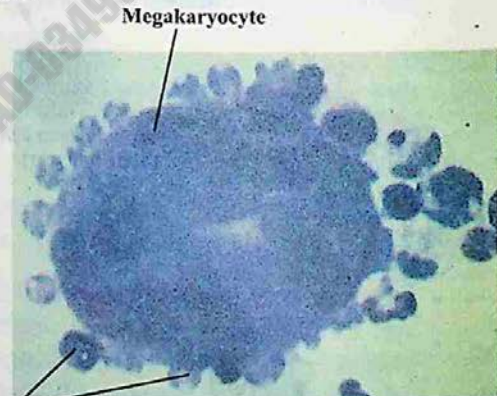
Platelets
