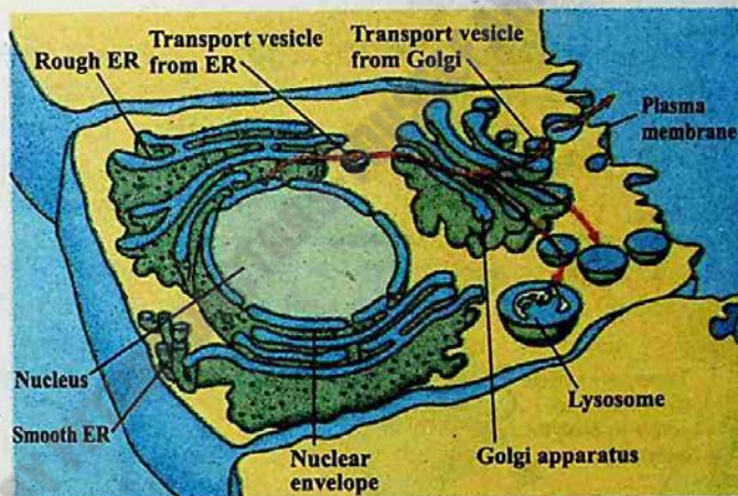
Fig. 4.9 Golgi Complex
