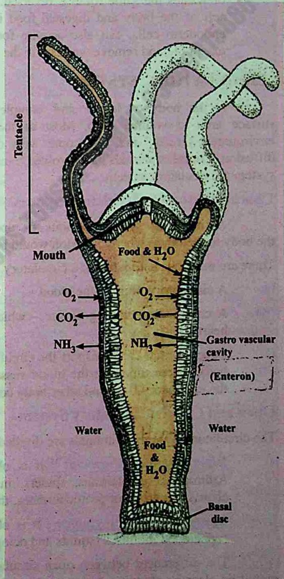
Fig.14.14 Hydra
