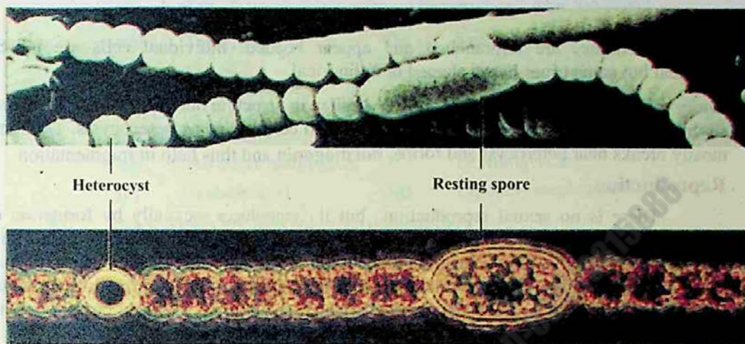
Fig. 6.8 Cyanobacterium Anabaena
