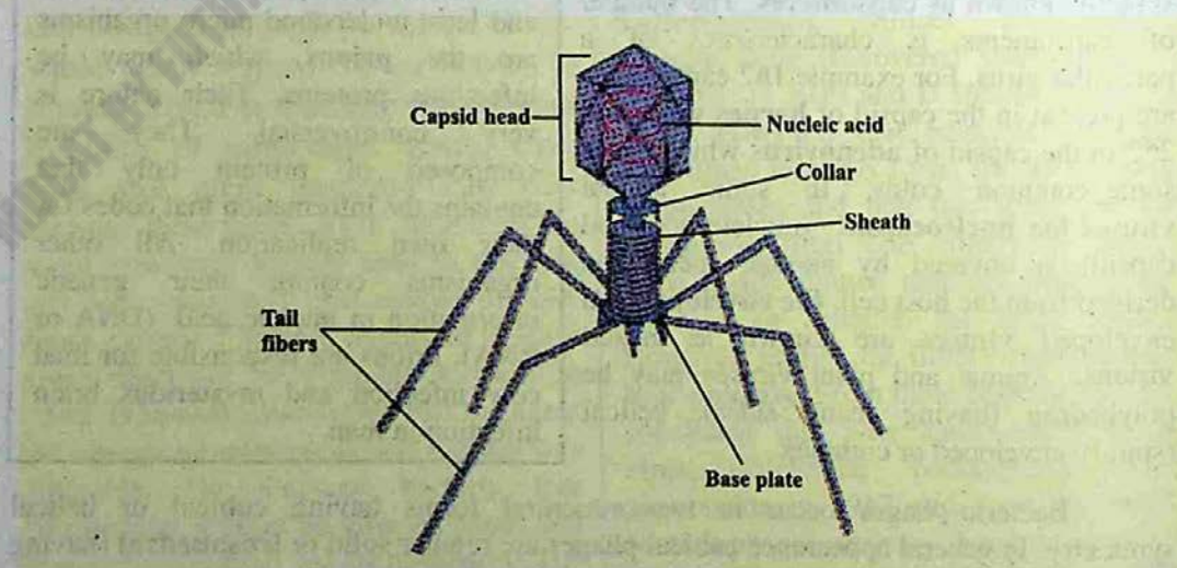
Fig. 5.4 A Bacteriophage
