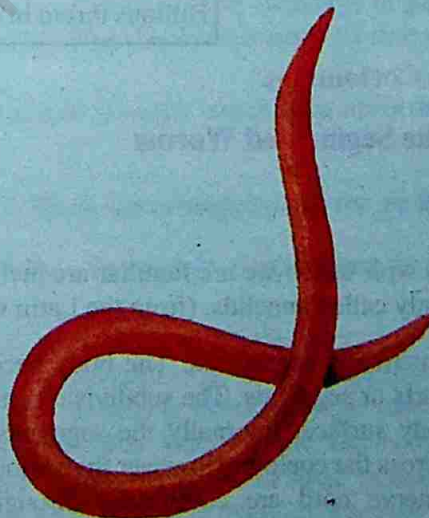
Roundworm
