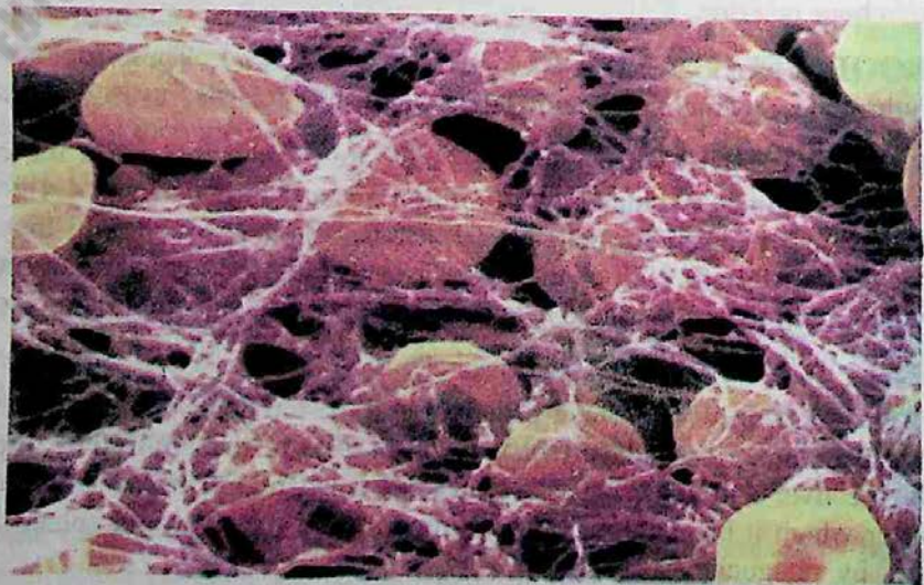
Fig.14.23 Blood clotting
