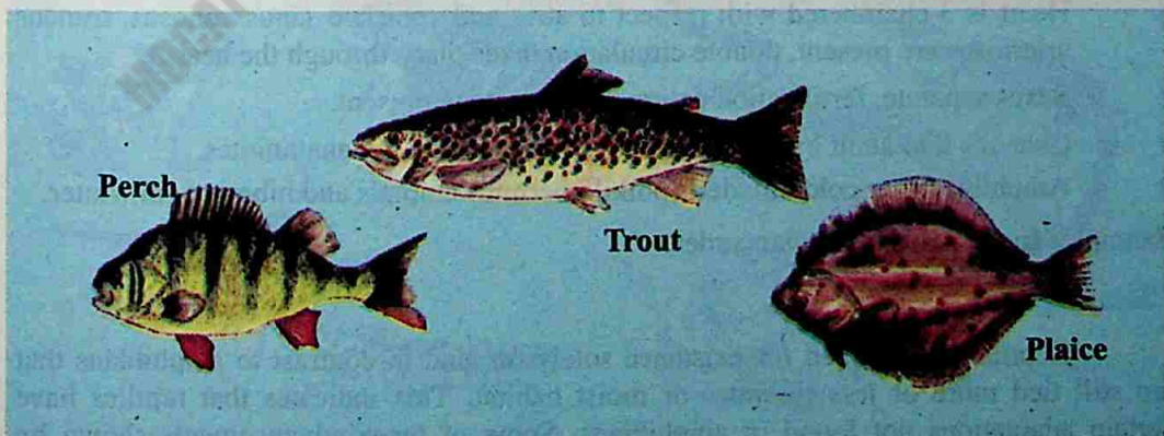
Fig. 10.17 Bony fishes
