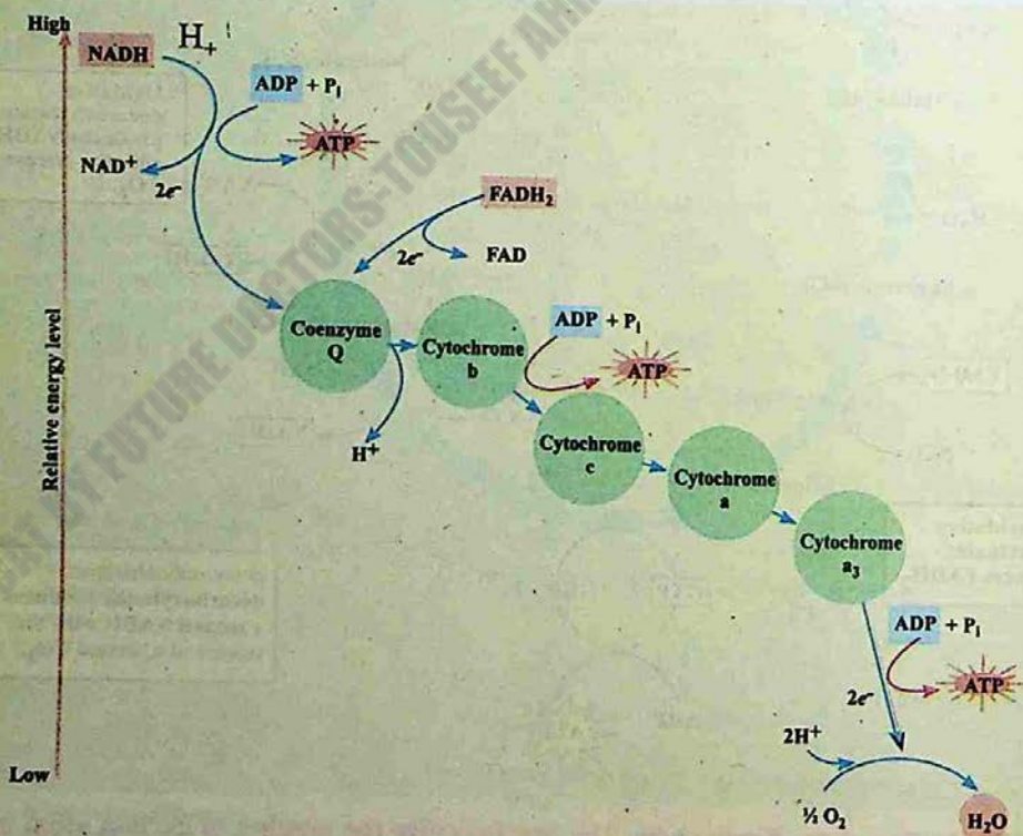
Fig. 11.14 The respiratory electron transport chain and its coupling with oxidative phosphorylation.
