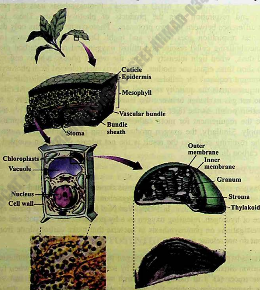
Fig. 11.1 A plant possesses thick layer of mesophyll cells rich in chloroplasts. Thylakoids in chloroplasts are stacked into grana. Light reactions take place on the grana, and dark reactions in the stroma.
